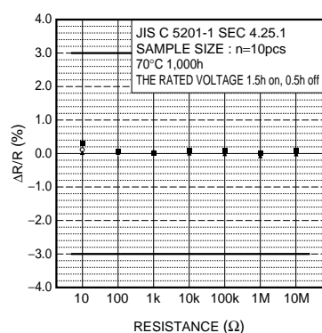
Fig.14 Endurance (at70°C)
