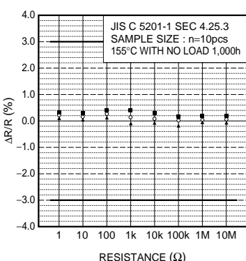
Fig.15 Endurance
