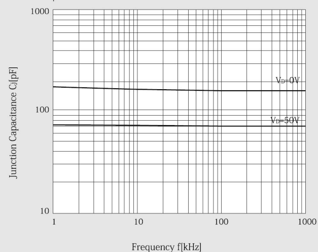
Junction Capacitance
