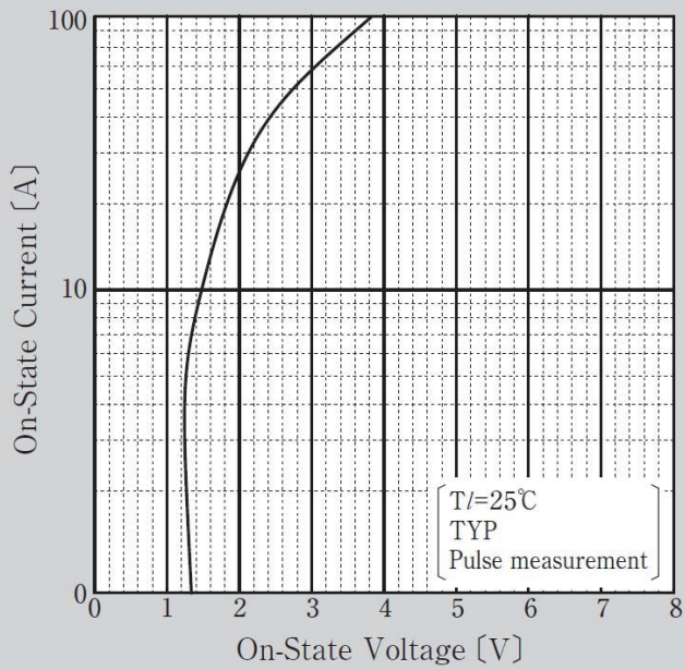
On-State Voltage-On-State Current
