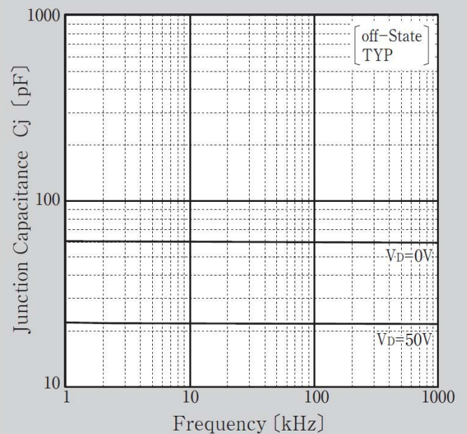
Junction Capacitance
