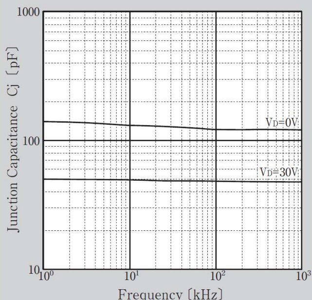
Junction Capacitance
