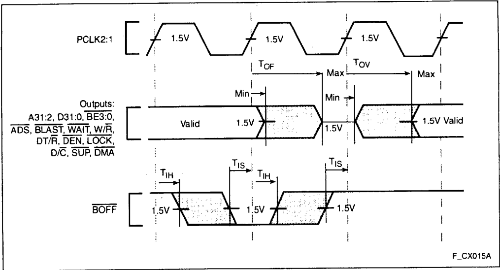
Figure 14. Bus Backoff (BOFF) Timings
