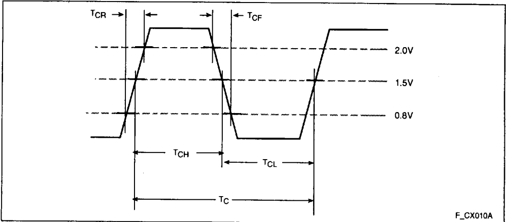
Figure 9. CLKIN Waveform
