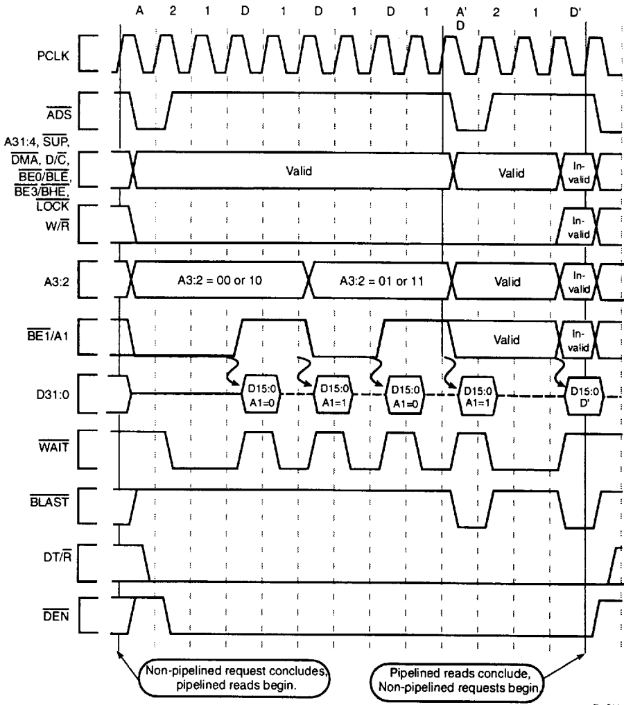
Figure 37. Burst, Pipelined Read Request With Wait States, 16-Bit Bus
