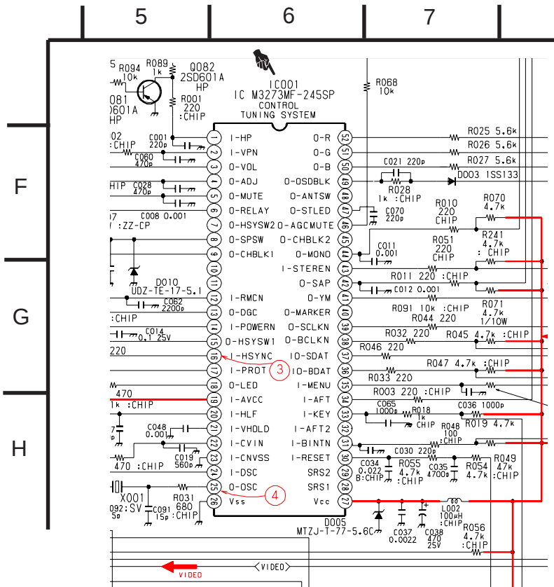
A BOARD PWB PART NO. 1-873-185-11
