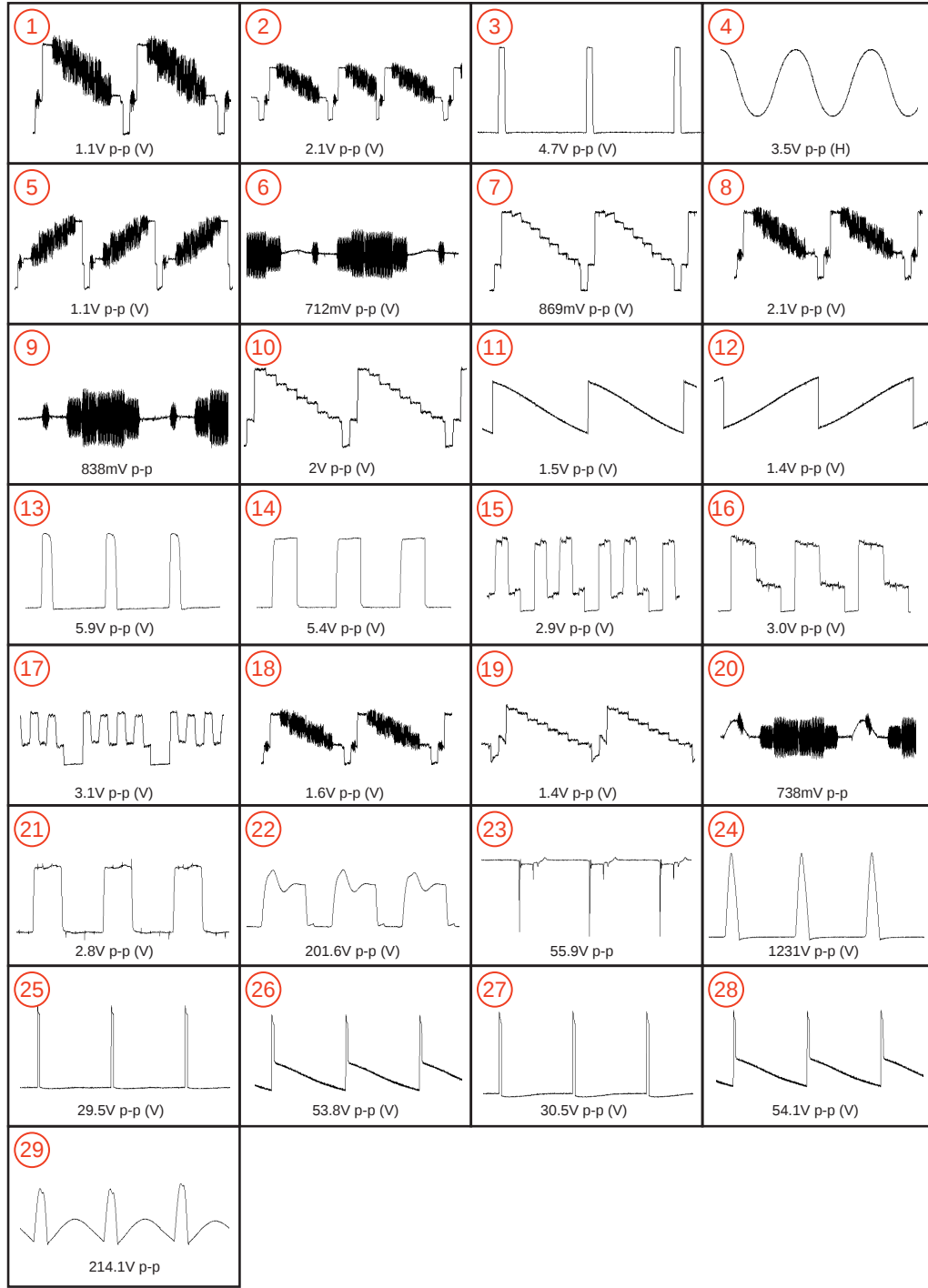
A BOARD WAVEFORMS
