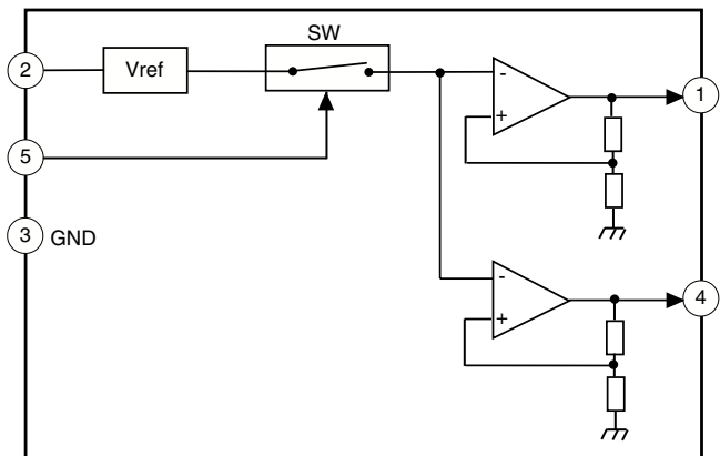
A BOARD IC601 MCZ3001D
