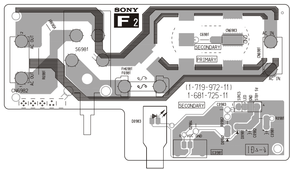
~ F2 Printed Wiring Board Conductor side ~
