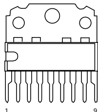
TDA6111Q/N4
