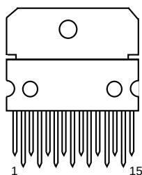
TDA7497
