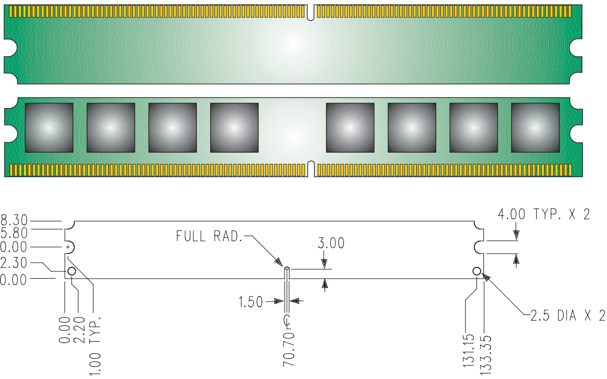
Figure 1: KVR800D2N5/1G 240-Pin DIMM
