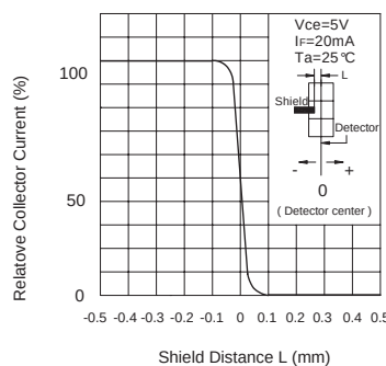
Fig.10 Relative Collector Current vs. Shield Distance (1)
