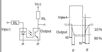
Test Circuit for Response Time
