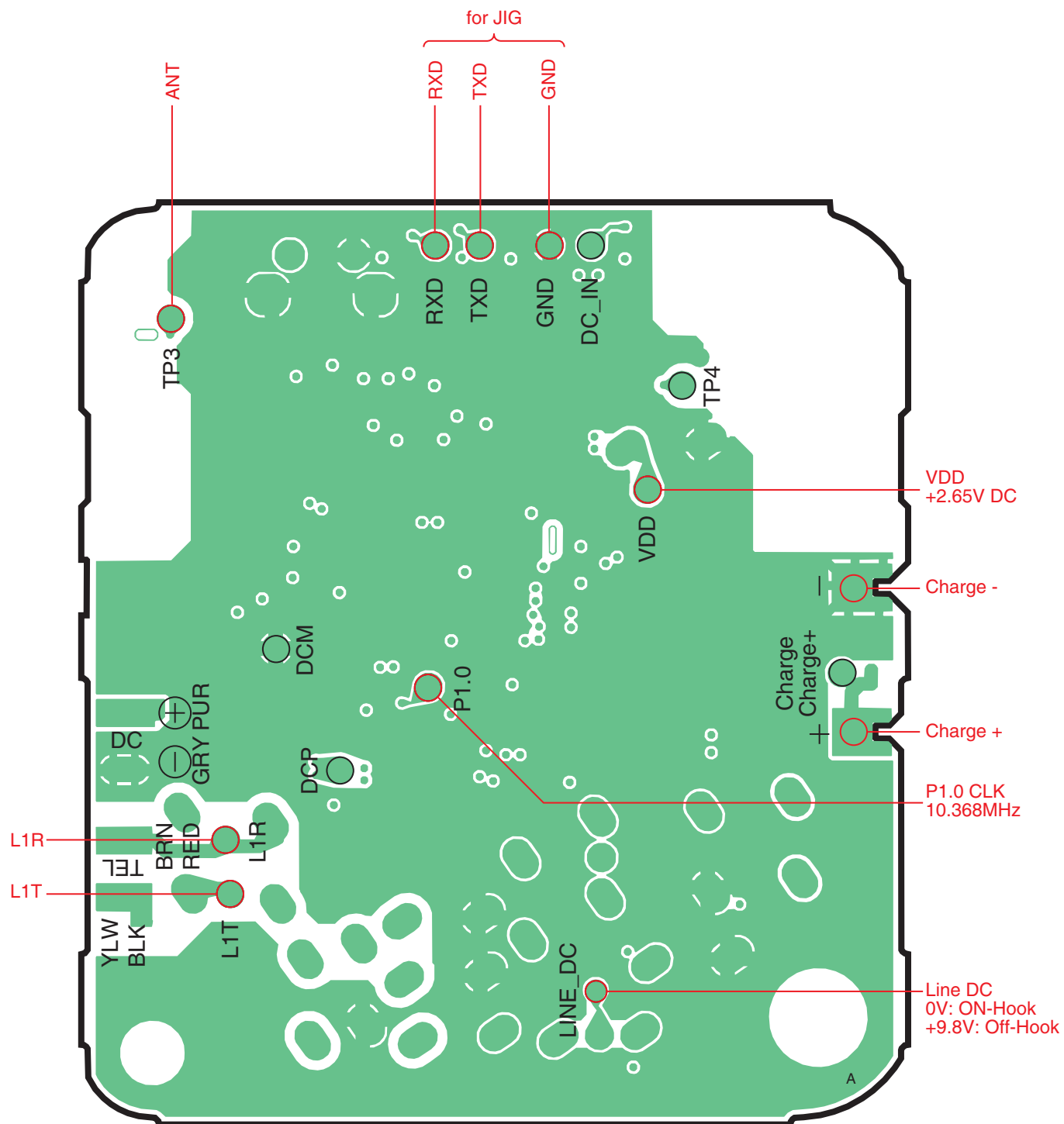
KX-TG1711/1712 CIRCUIT BOARD (Base Unit_Main (Bottom View))
