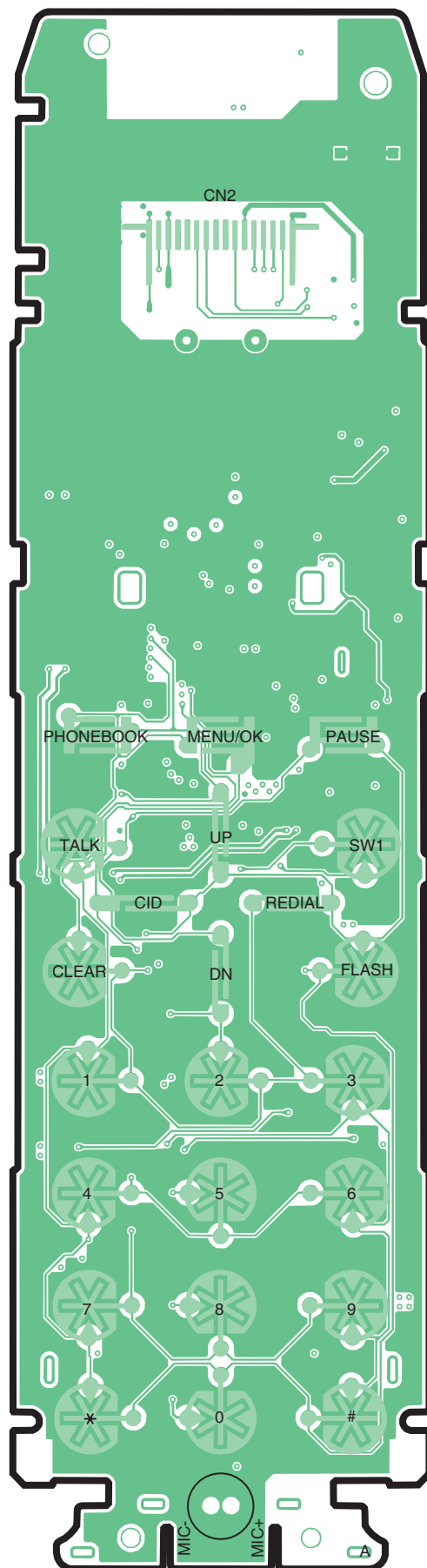
KX-TGA171 CIRCUIT BOARD (Handset_Main (Bottom View))
