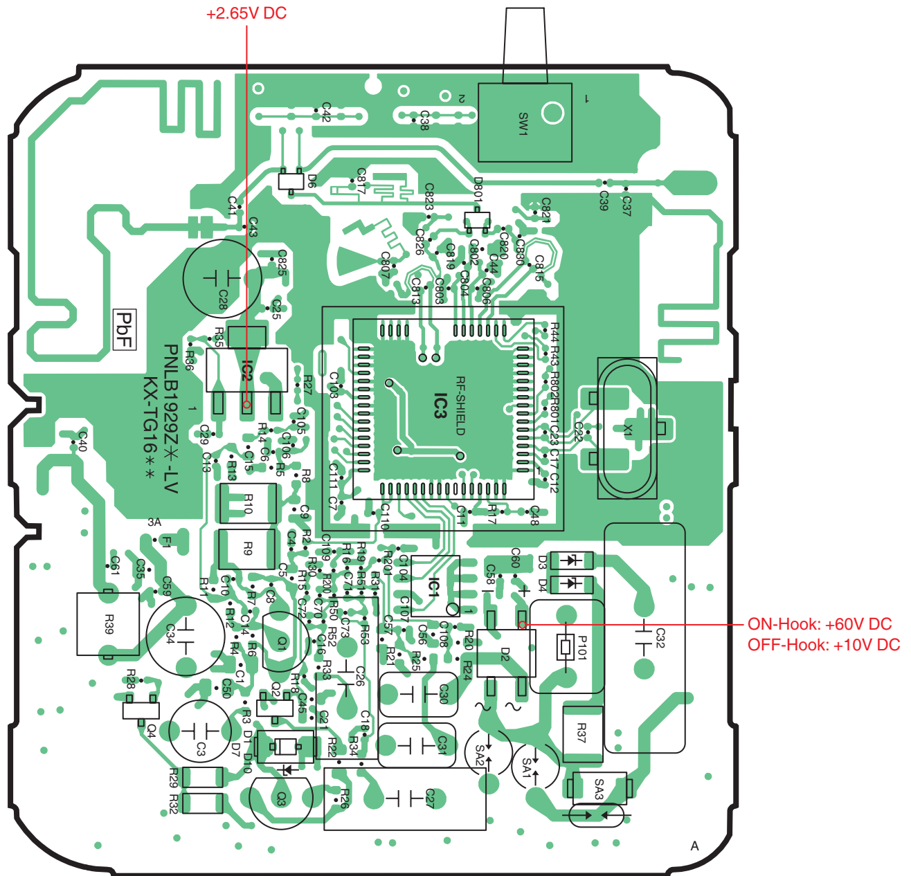
KX-TG1711/1712 CIRCUIT BOARD (Base Unit_Main (Component View))
