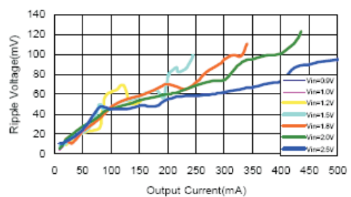
KX8530-331SM Ripple Voltage VS. Output Current
