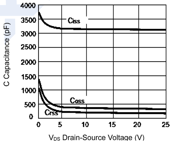
Figure10. Capacitance
