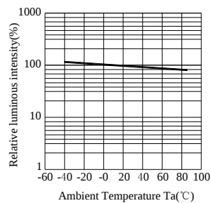
Fig.5 Luminous Intensity vs. Ambient Temperature
