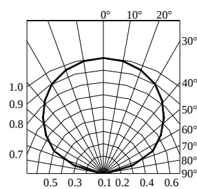
Fig.7 Relative Intensity vs. Angle
