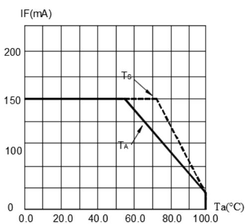
FIG. 2 MAXIMUM FORWARD DC CURRENT VS AMBIENT TEMPERATURE ( T_{jmax}=120\text{ }^{\circ}\text{C} ) T_A temp. ambient; T_s temp. solder point.
