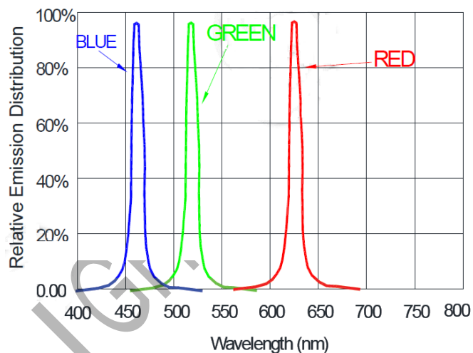
Wavelength Characteristics
