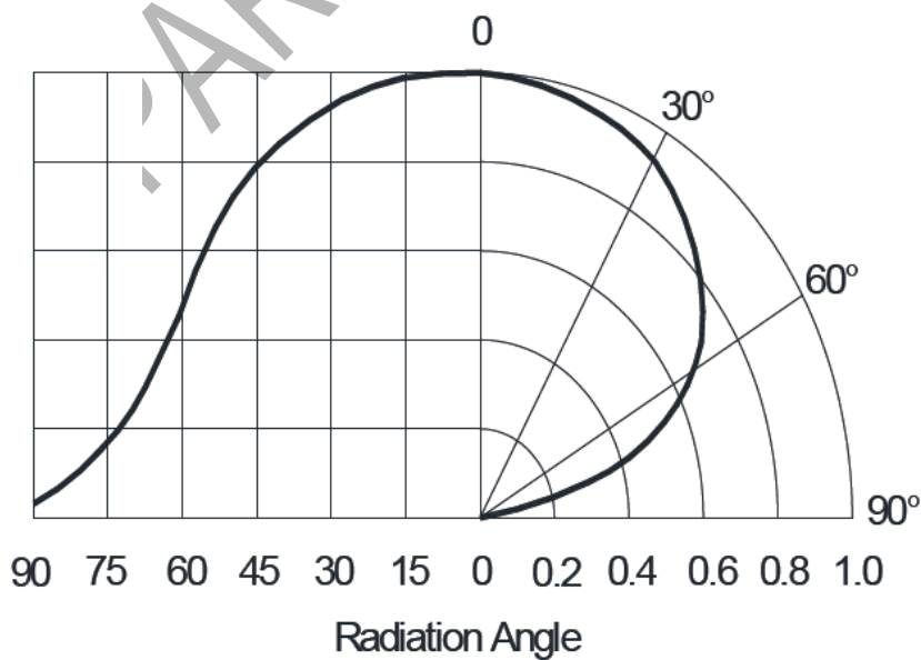
Typical Radiation Pattern 120°
