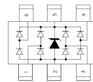
4 lines Protection
