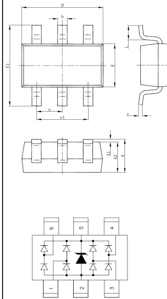
4 lines Protection
