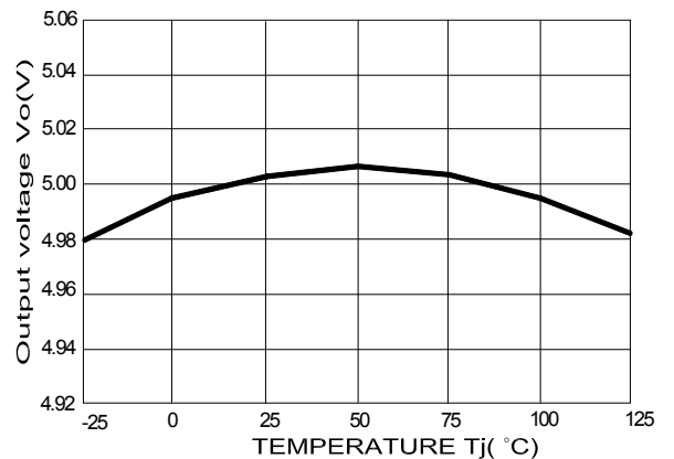
Output Voltage vs. Temperature(Tj)(L1481T-5)
