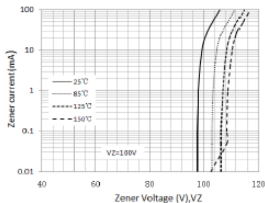
Figure 1. Typical Zener Voltage, V_Z=100\text{V}
