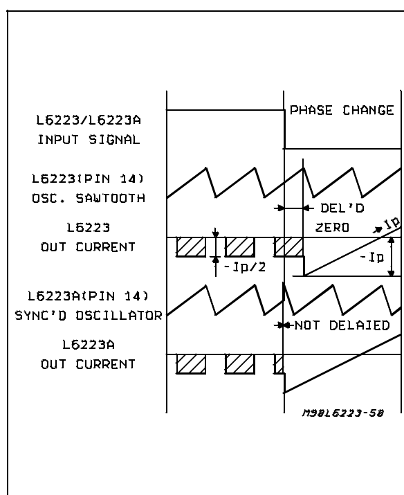
Figure 21b: Oscillator behaviour of the L6223 and of the L6223 (simplified waveforms).
