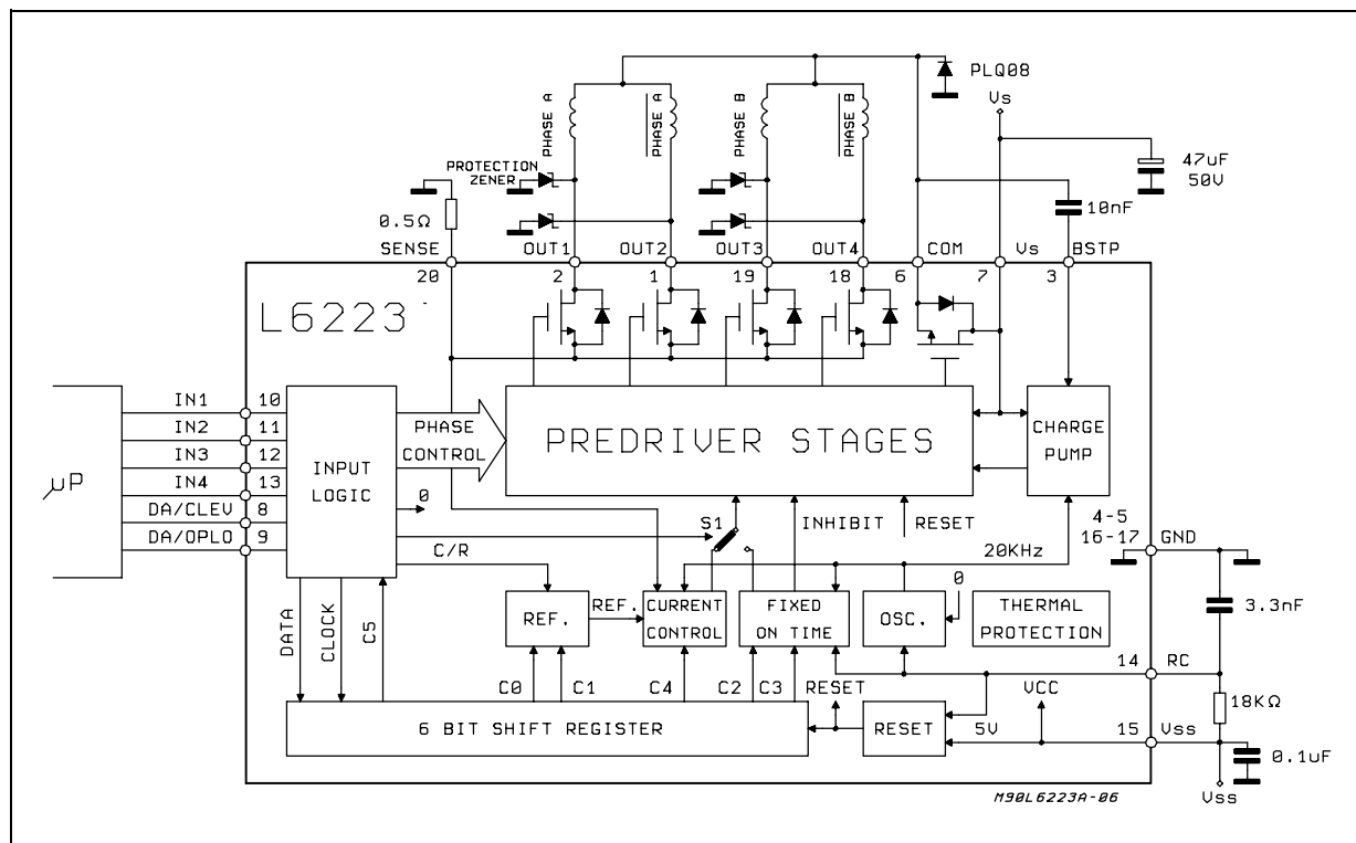
Figure 10: Typical Application Circuit using a single device: the max peak current capability is of 1A/phase ( R_s = 0.25\Omega )
