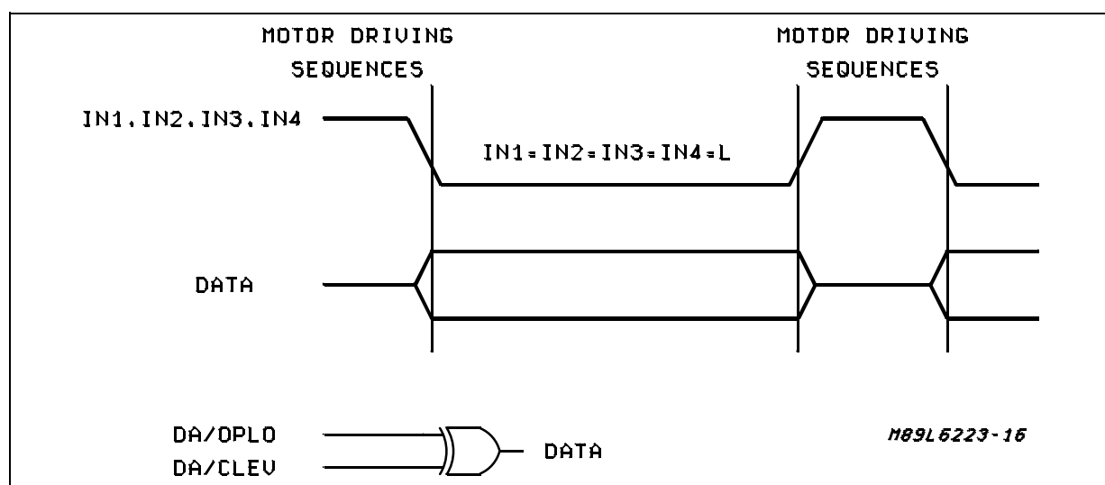
Figure 9: Waveform for programming: the output is disabled only when all four inputs are at the low level.
