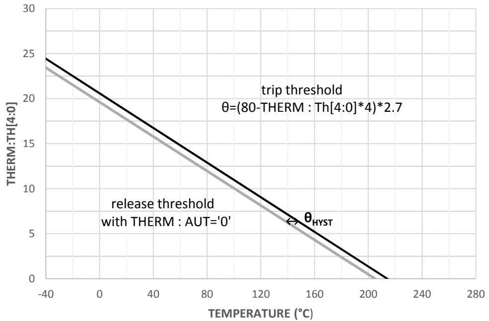
Figure 12. L6364 thermal shutdown configuration
