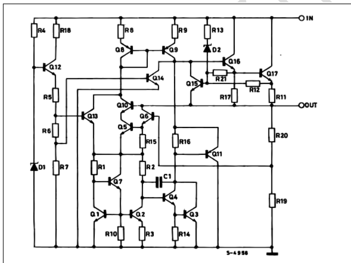
Figure 3. Schematic diagram
