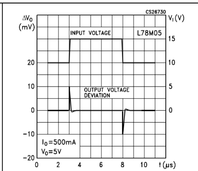
Figure 15. Line transient response
