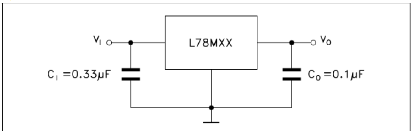
Figure 4. Application circuit
