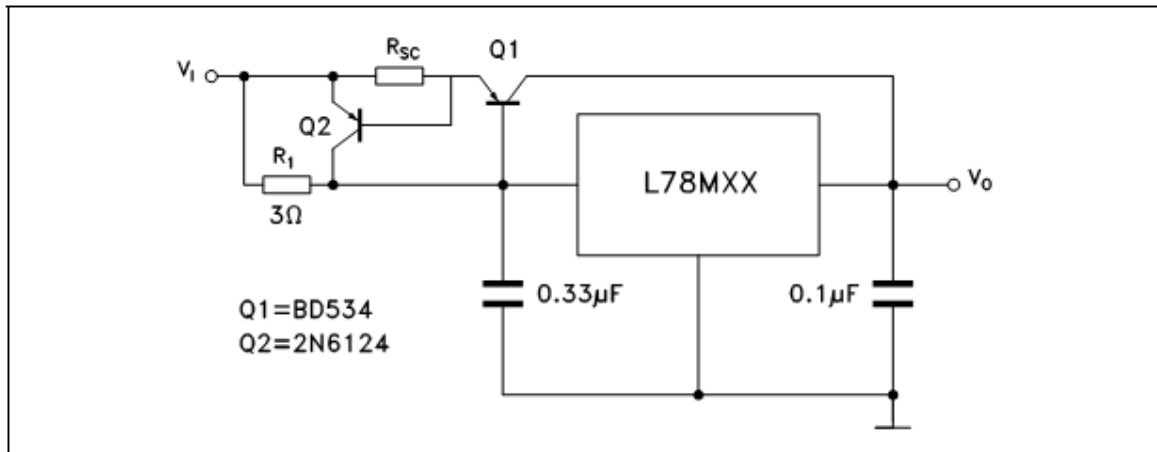
Figure 20. Short-circuit protection
