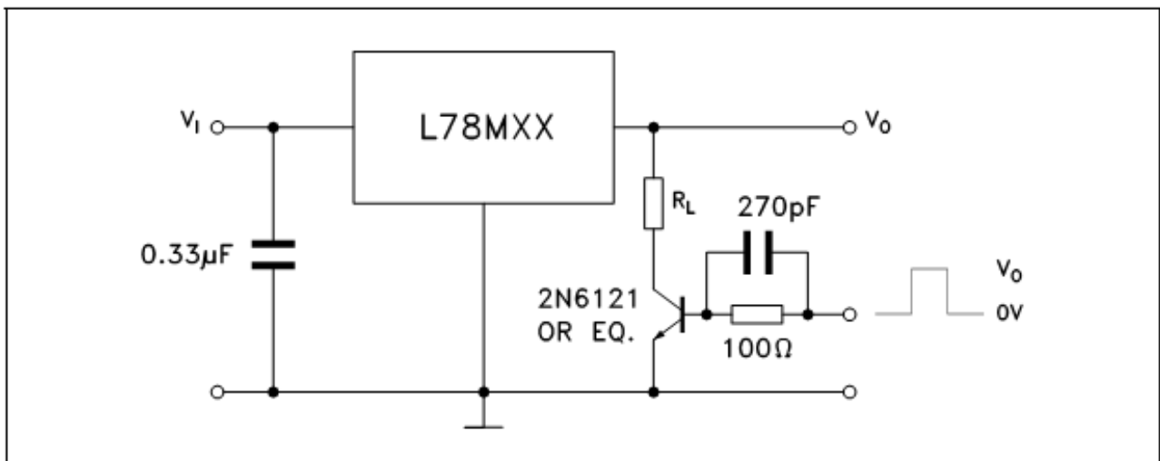
Figure 6. Load regulation
