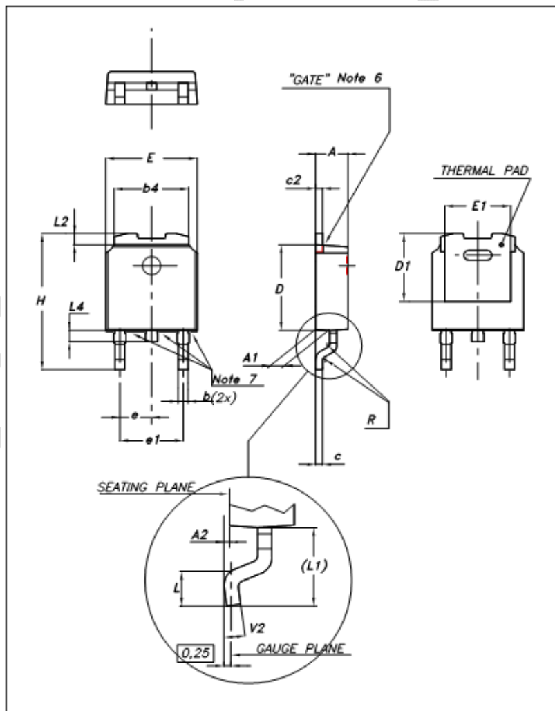
Figure 21. Drawing dimension DPAK
