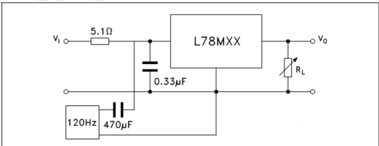
Figure 7. Ripple rejection
