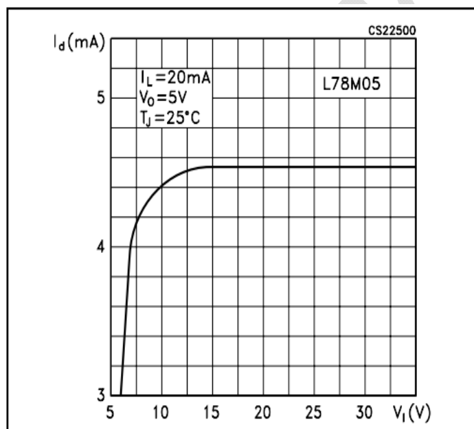
Figure 16. Quiescent current vs. input voltage
