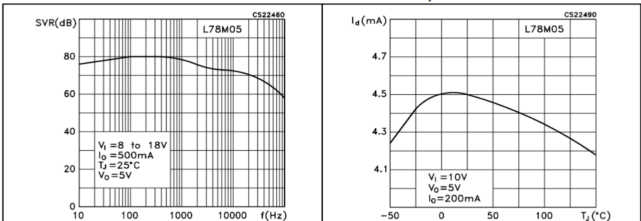
Figure 12. Supply voltage rejection vs. freq. Figure 13. Quiescent current vs. junction temp.
