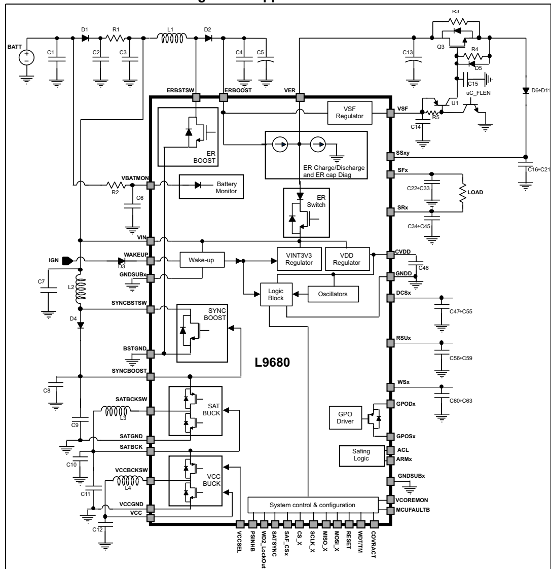
Figure 71. Application circuit
