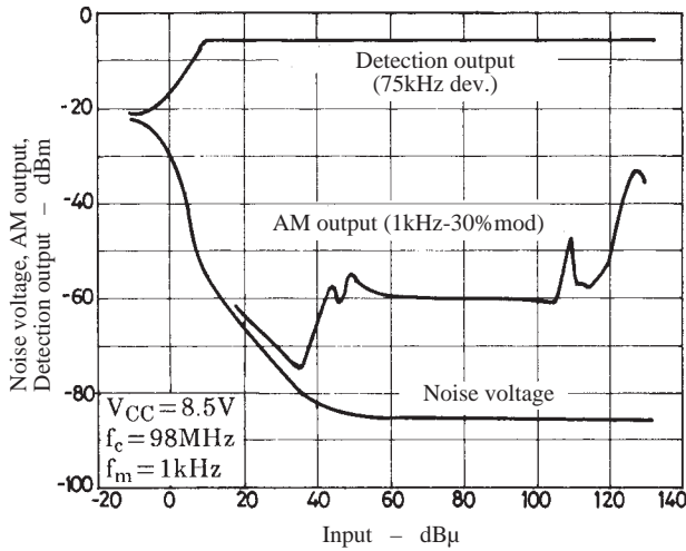
LA1177+LA1266 Overall Characteristic
