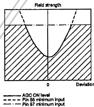
Figure 23. Wideband AGC and antenna input field strength
