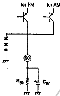
Figure 19. S-meter output
