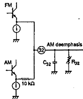
Figure 31. AM level
