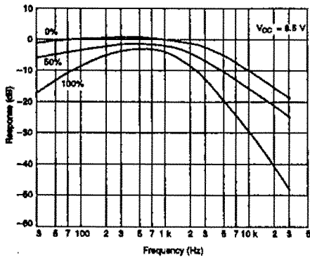
Low-pass filter frequency response (2)
