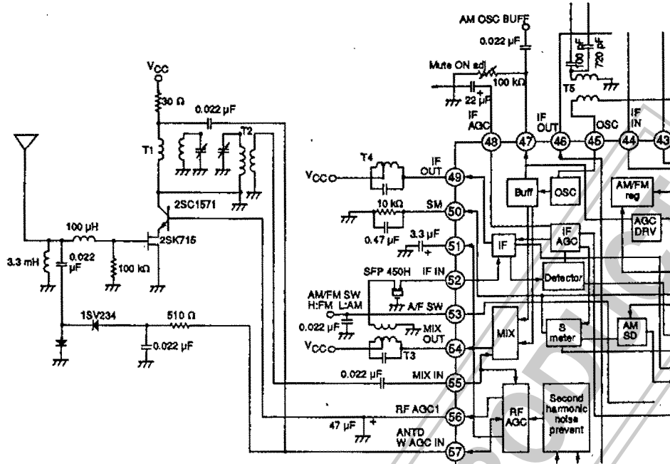
Figure 21. AGC stage
