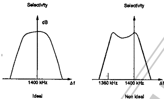
Figure 32. Tracking characteristic
