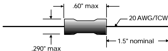
Dimensions include shrink tubing
