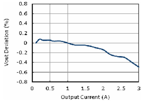
Load Regulation
