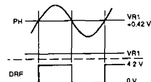
Figure 4. RF detector output
