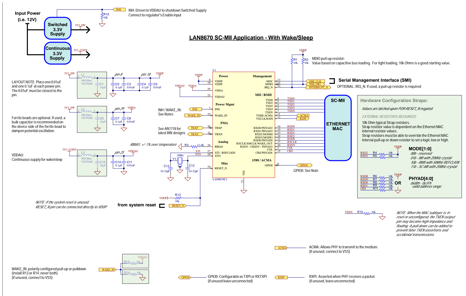
Figure 6-12. LAN8670 SC-MII Reference Schematic (With Sleep/Wake)
