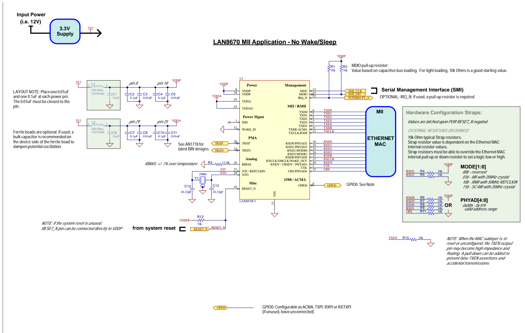
Figure 6-9. LAN8670 MII Reference Schematic (No Sleep/Wake)
