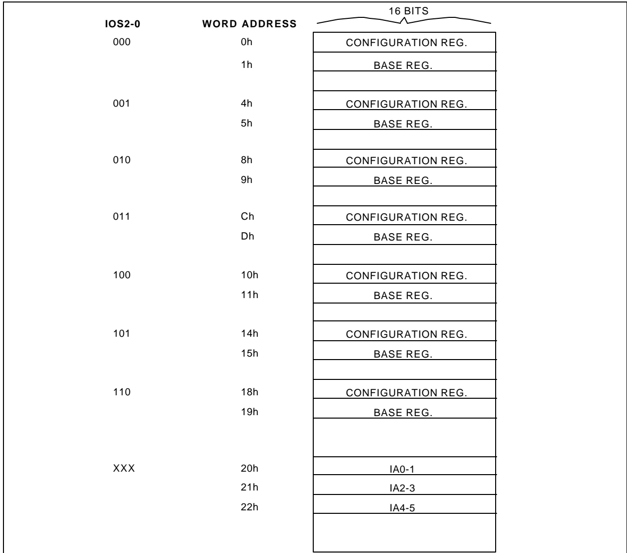
FIGURE 19 - 64 X 16 SERIAL EEPROM MAP
