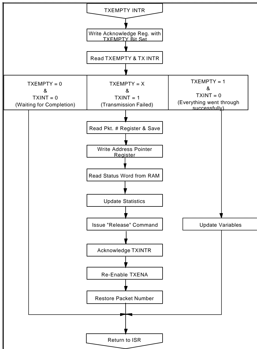
FIGURE 15 -TXEMPTY INTR (Assumes Auto Release Option Selected)
