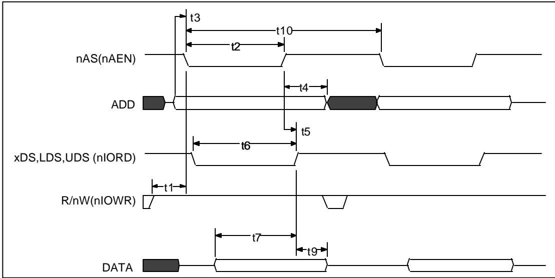
FIGURE 29 - 68000 READ TIMING
