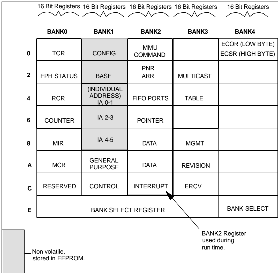
FIGURE 10 - LAN91C96 REGISTERS
