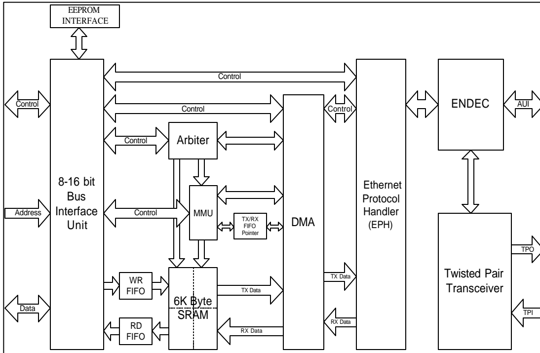
FIGURE 7 - LAN91C96 INTERNAL BLOCK DIAGRAM WITH DATA PATH
