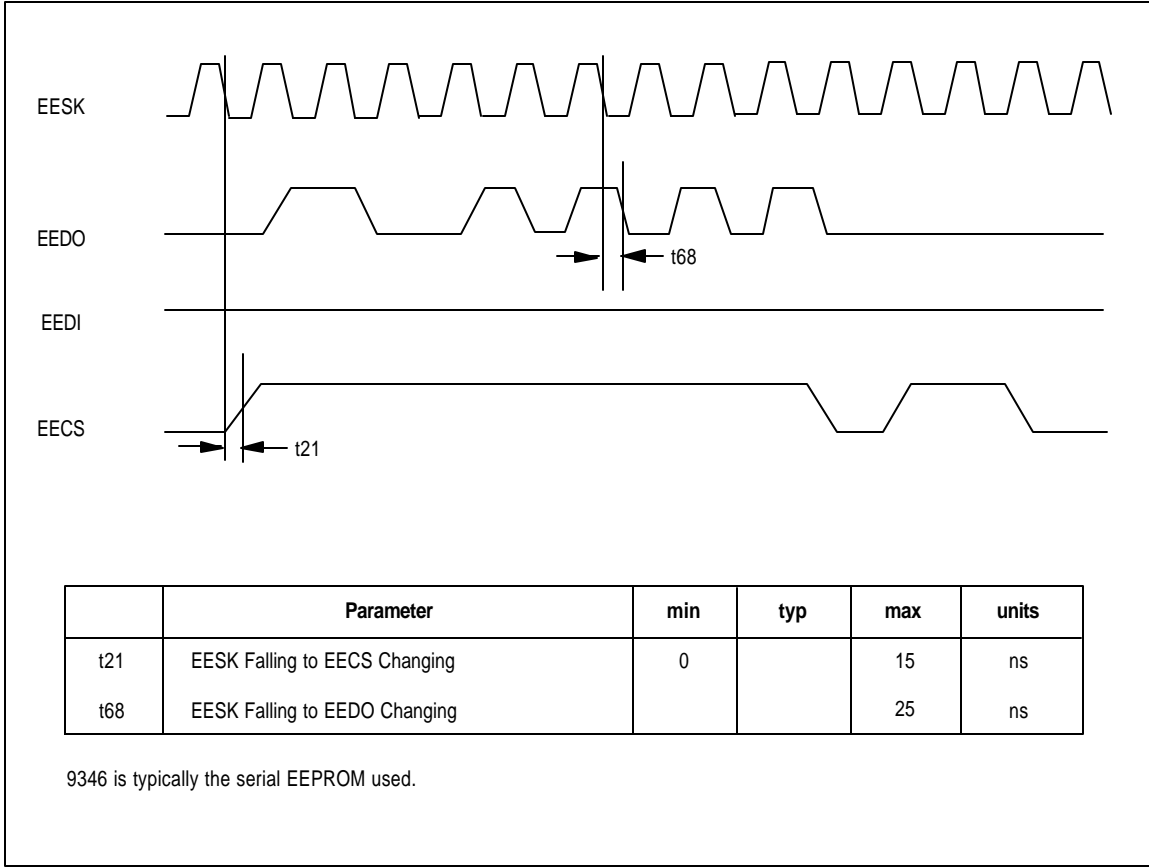
FIGURE 34 - EEPROM READ
