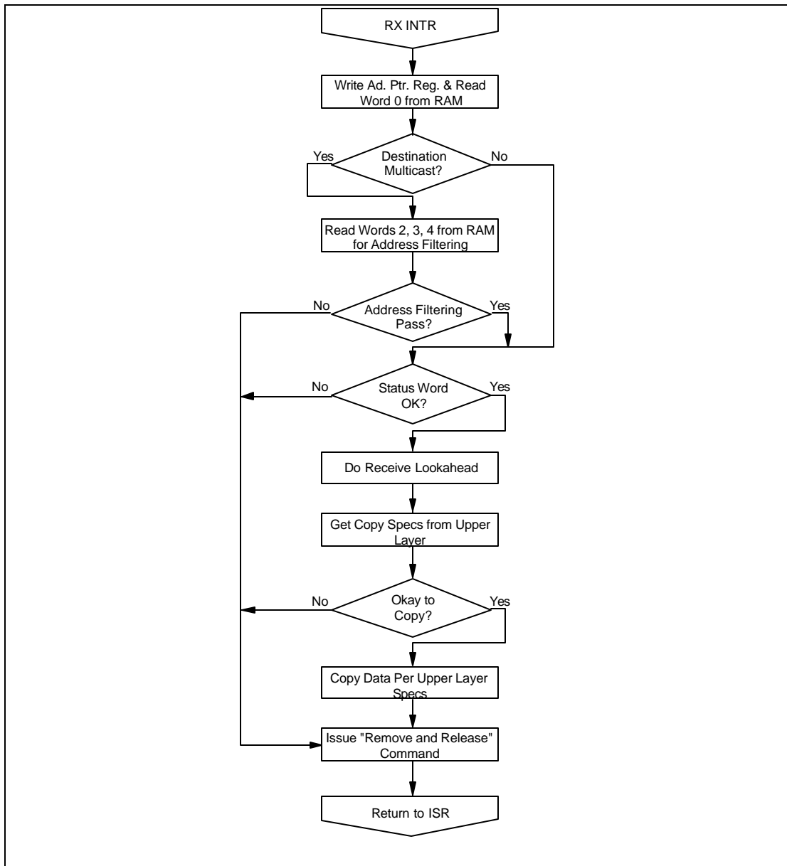
FIGURE 13 - RX INTR
