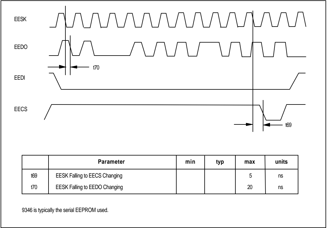
FIGURE 35 - EEPROM WRITE
