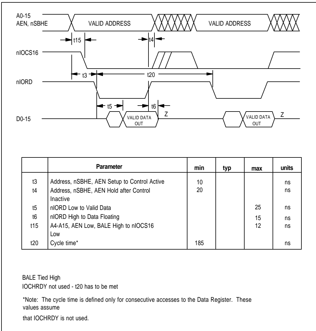
Figure 21 - LOCAL BUS CONSECUTIVE READ CYCLES
