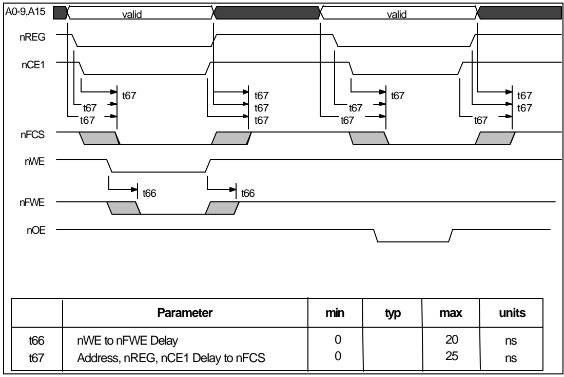
FIGURE 36 - PCMCIA ATTRIBUTE MEMORY READ/WRITE (A15=0)
