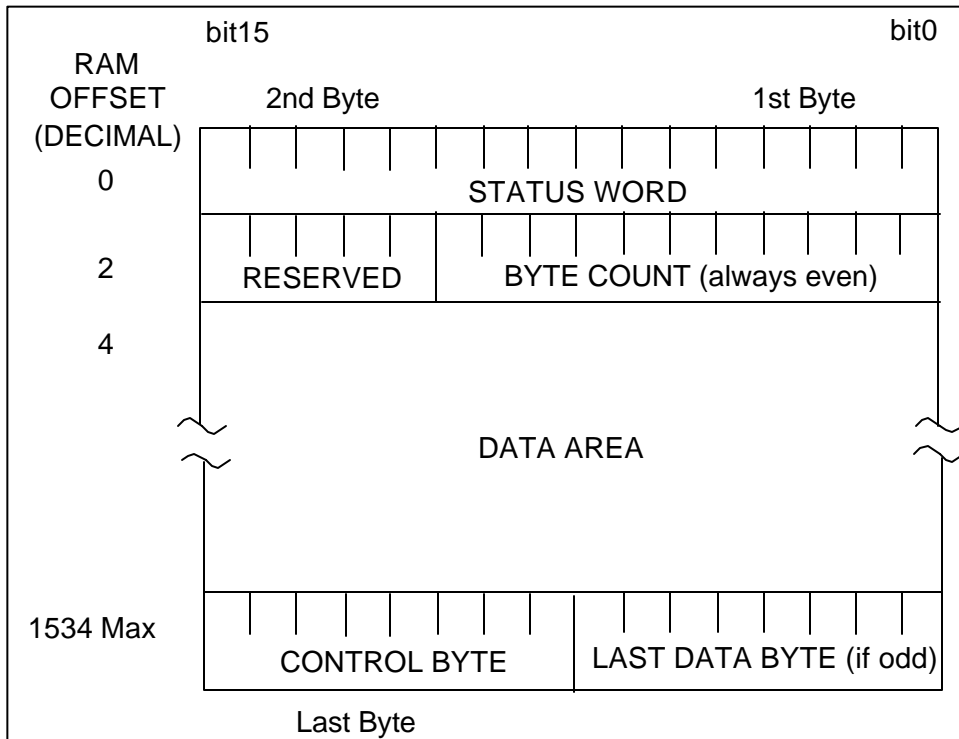
FIGURE 9 - DATA FRAME FORMAT
