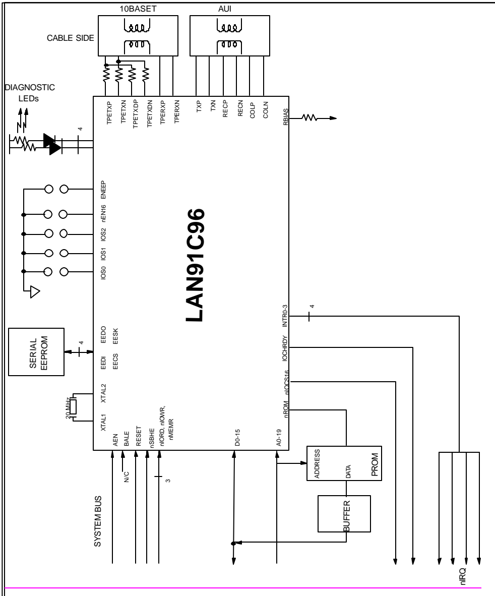
FIGURE 2 - SYSTEM DIAGRAM FOR LOCAL BUS WITH BOOT PROM
