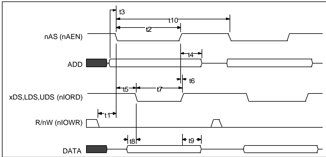
FIGURE 30 - 68000 WRITE TIMING
