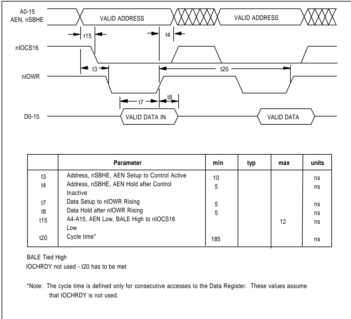
FIGURE 23 - LOCAL BUS CONSECUTIVE WRITE CYCLES
