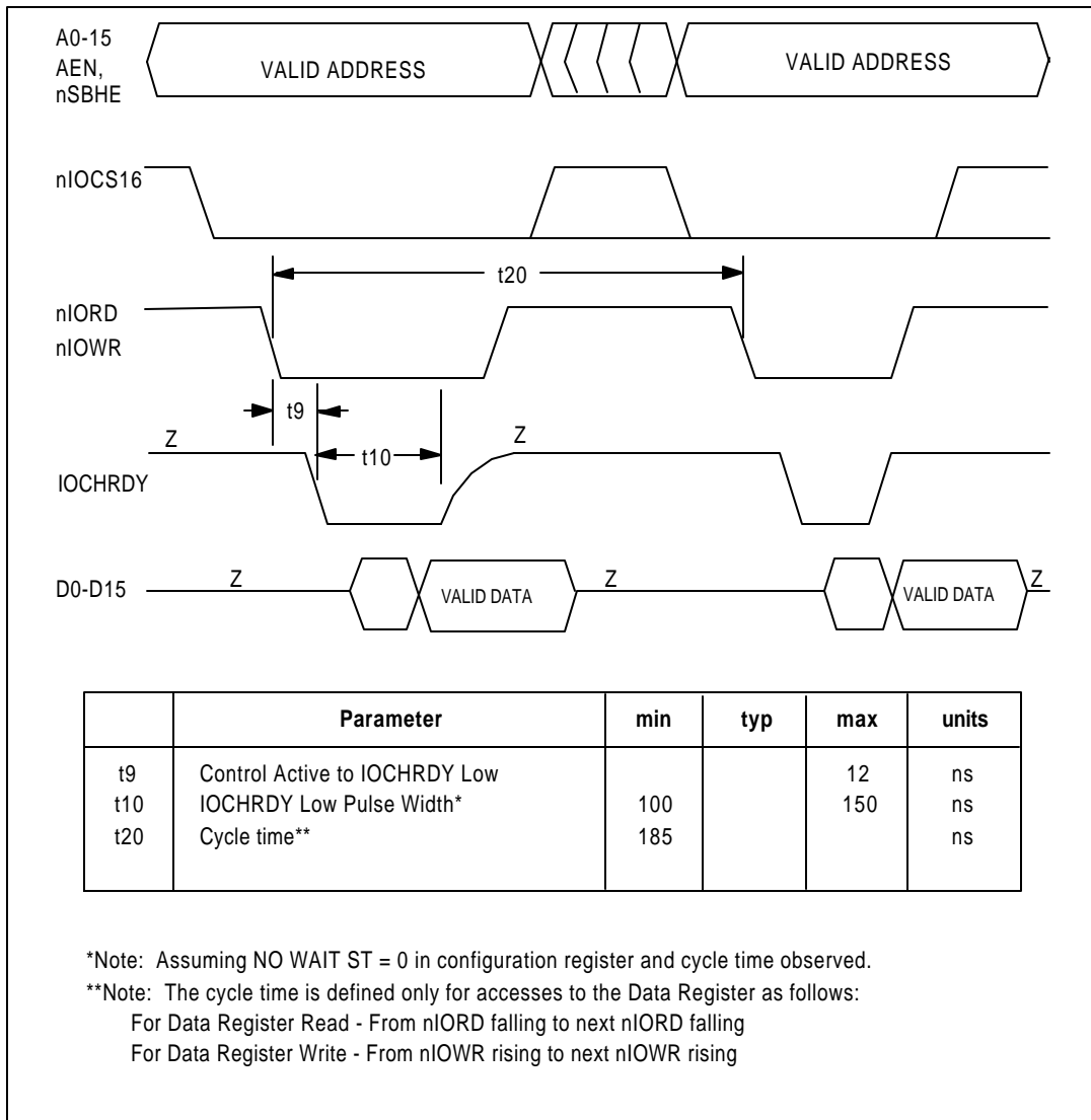
FIGURE 25 - LOCAL BUS CONSECUTIVE READ AND WRITE CYCLES
