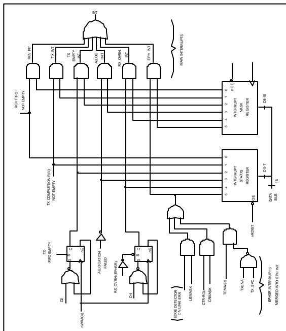
FIGURE 11 - INTERRUPT STRUCTURE
