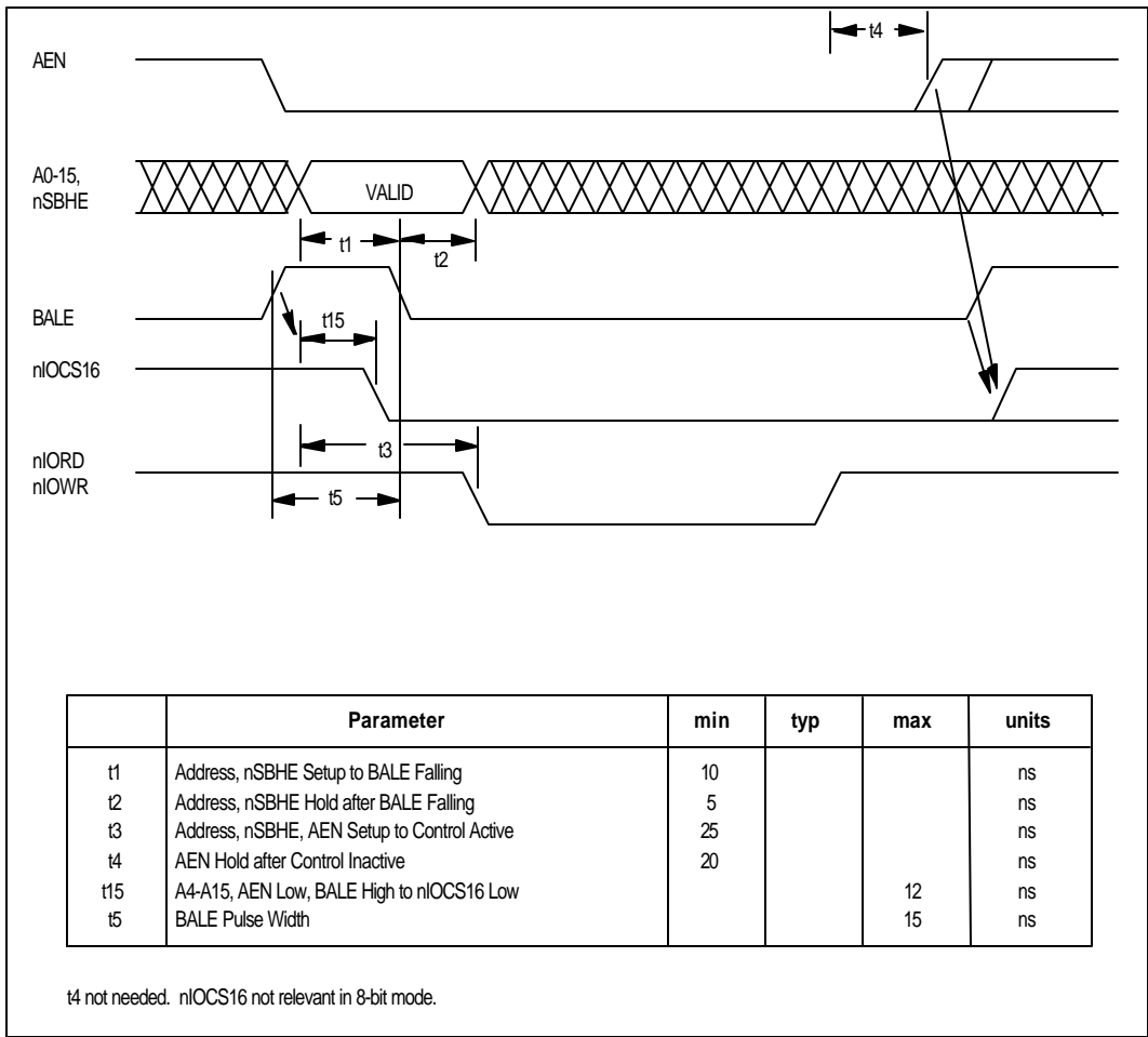
FIGURE 32 - LOCAL BUS REGISTER ACCESS WHEN USING BALE
