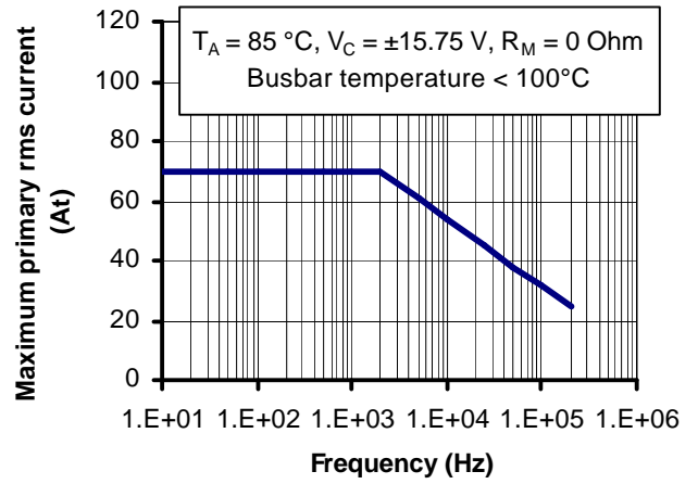
Figure 3: Frequency derating
