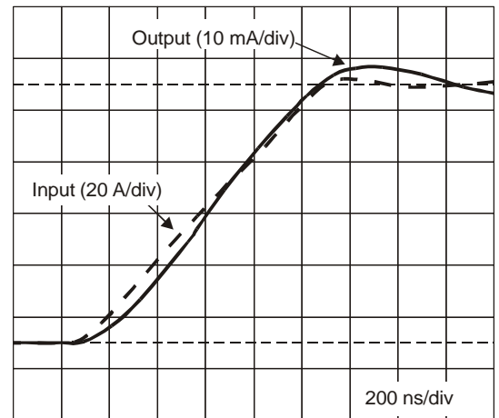
Figure 15: Typical di/dt follow-up (high speed 1 turn PCB design)
