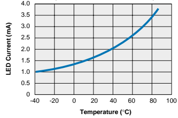
LBA127L - Form B Typical I F for Switch Dropout vs. Temperature (Load Current = 170mADC)
