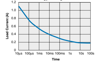
LBA127L Energy Rating Curve
