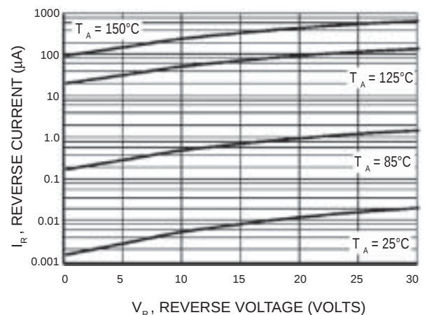
Figure 3. Leakage Current
