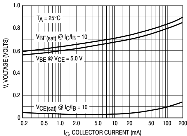
Figure 2. "On" Voltage
