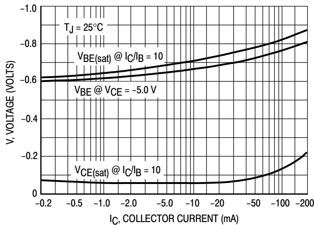
Figure 8. "On" Voltage
