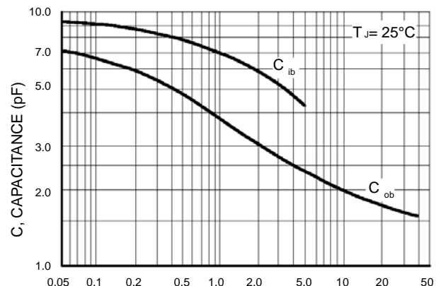
Figure 13. Capacitance
