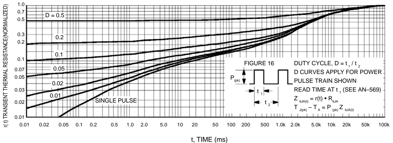
Figure 14. Thermal Response
