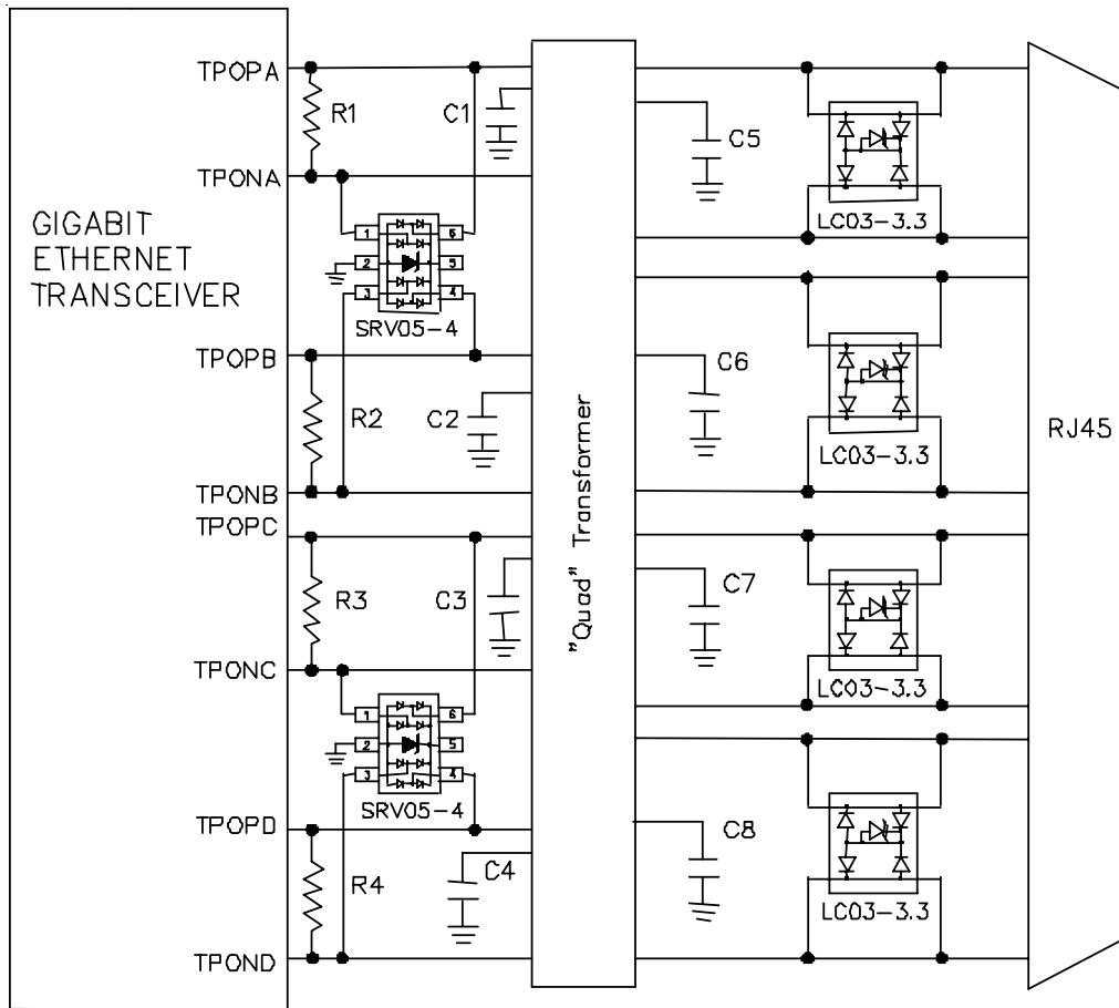
Bellcore 1089 Intra-Building Protection Gigabit Ethernet
