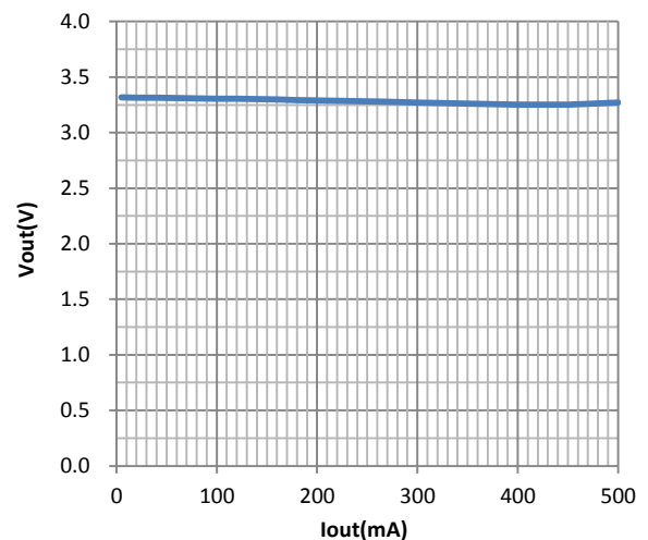
Load Regulation
