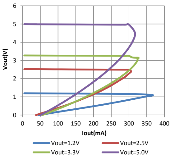
Current Limit
