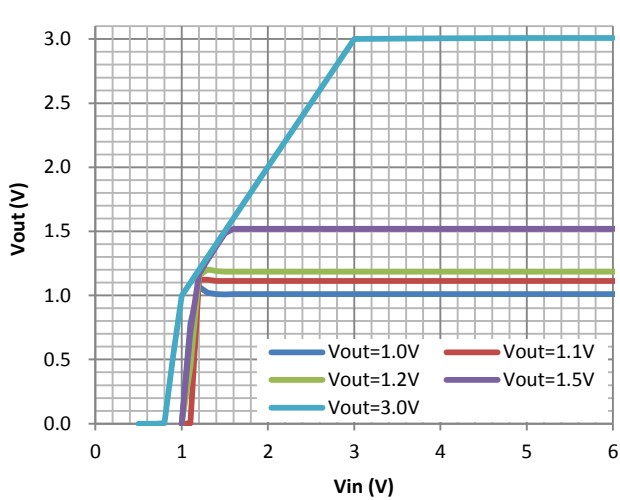
Line Regulation
