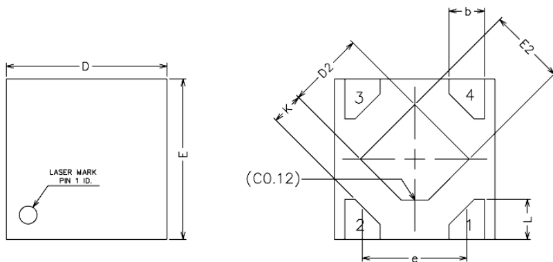
COMMON DIMENSIONS (UNITS OF MEASURE=MILLIMETER)
