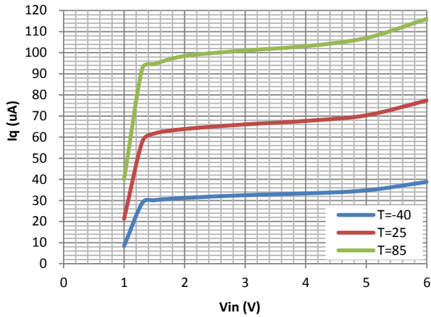
Iq (Vout=1V)
