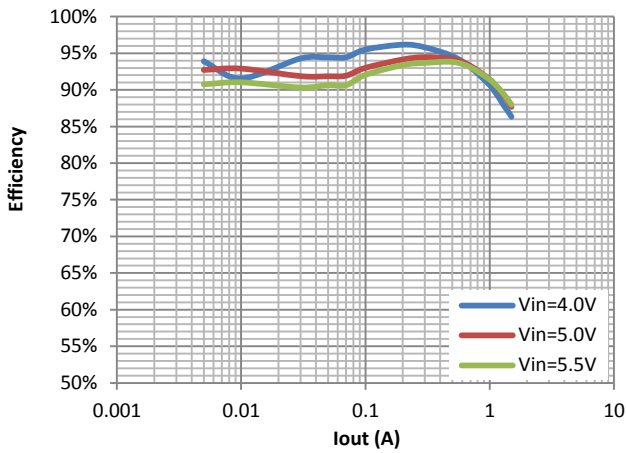
Efficiency vs. Output Current ( V_{out}=3.3\text{V} )
