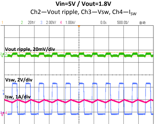
Output Ripple and SW at 1A load
