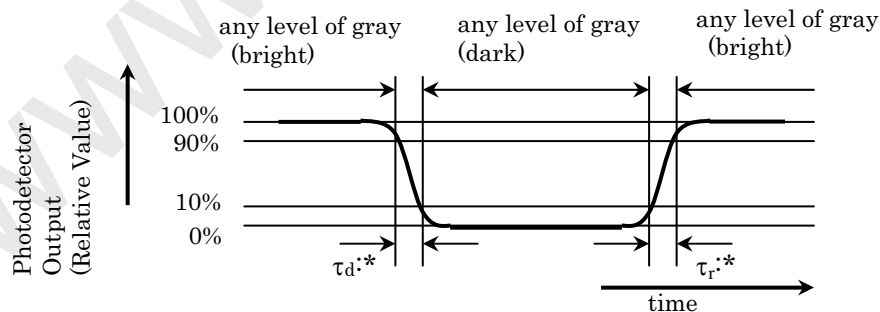
Fig.9-4 Response time
