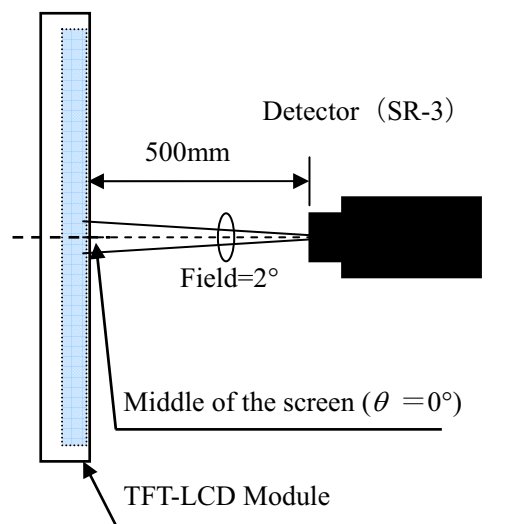
Fig.9-2 Measurement of Contrast, Chromaticity, White variation.
