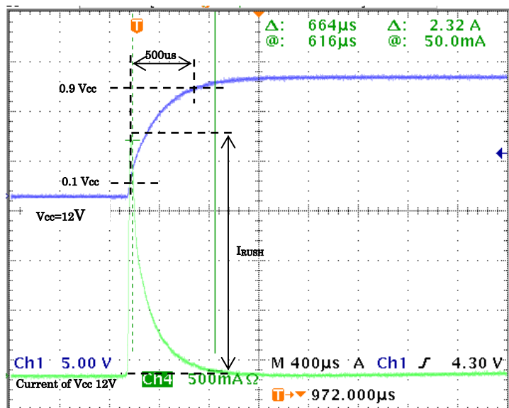
Fig. 6-5 The waveform of rush current
