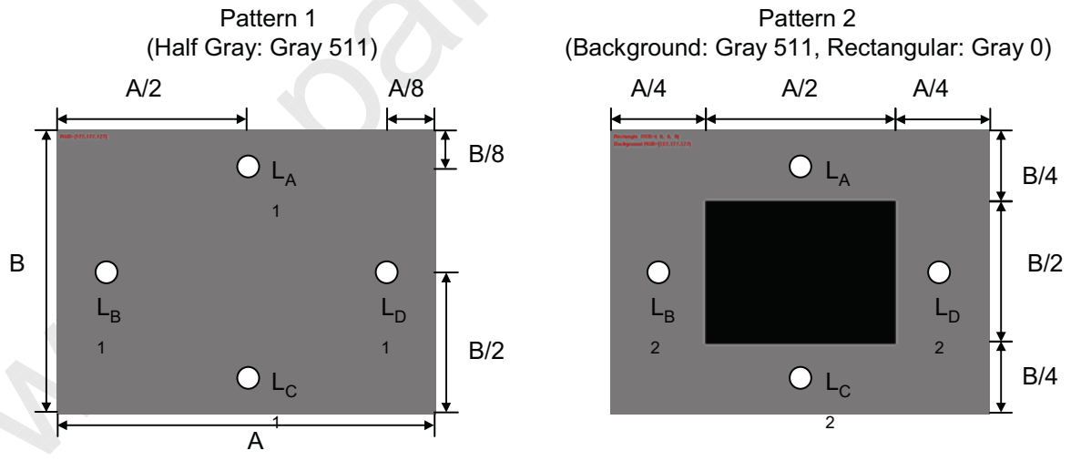
FIG. 5 Cross Talk
