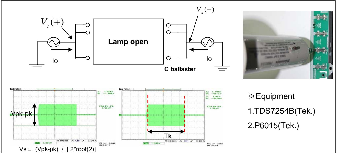
Figure 1 . EEFL Vopen
