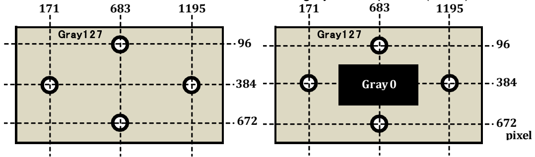
Fig.9-6 measurement locations of Y_A
