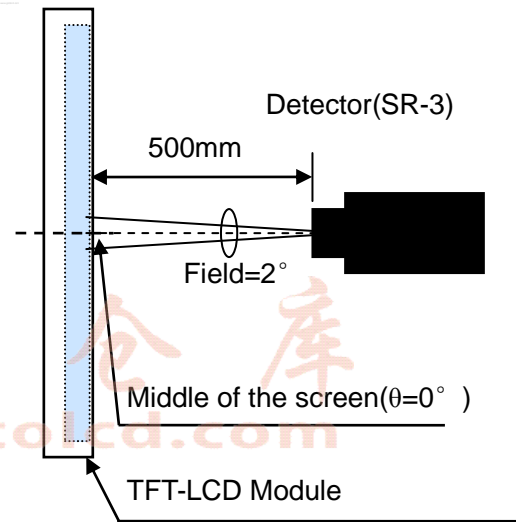
Fig.9-2 Measurement of Contrast, Luminance, Chromaticity, White variation
