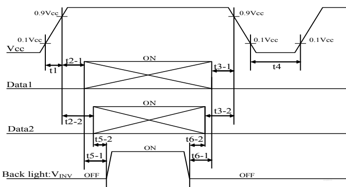
Fig. 6-1 Input voltage sequences
