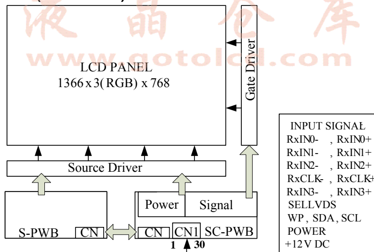
Fig.5-3 block diagram (Open-cell)
