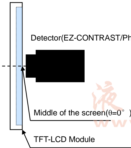
Fig.9-1 Measurement of Viewing angle range and Response time. (Viewing angle range: EZ-CONTRAST, Response time: Photodiode)
