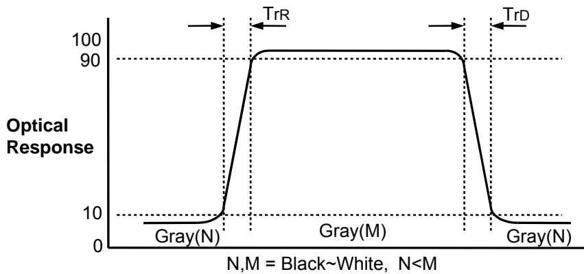
FIG. 10 Response Time
