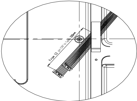
Detail A Scale 1:1.5
