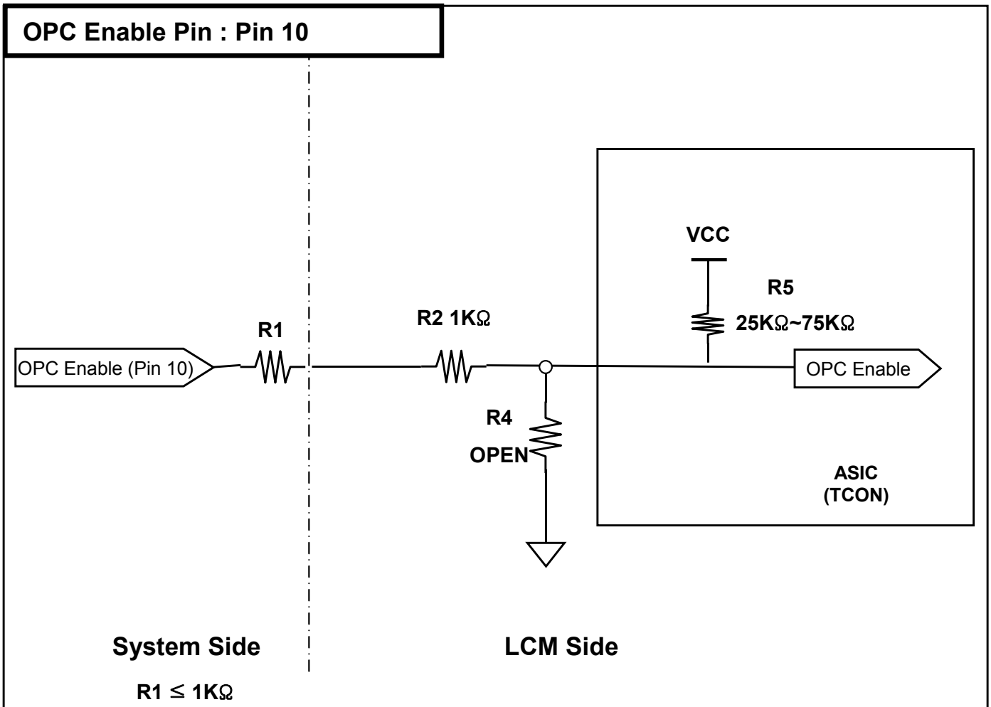
Circuit Block Diagram of OPC Enable Selection pin
