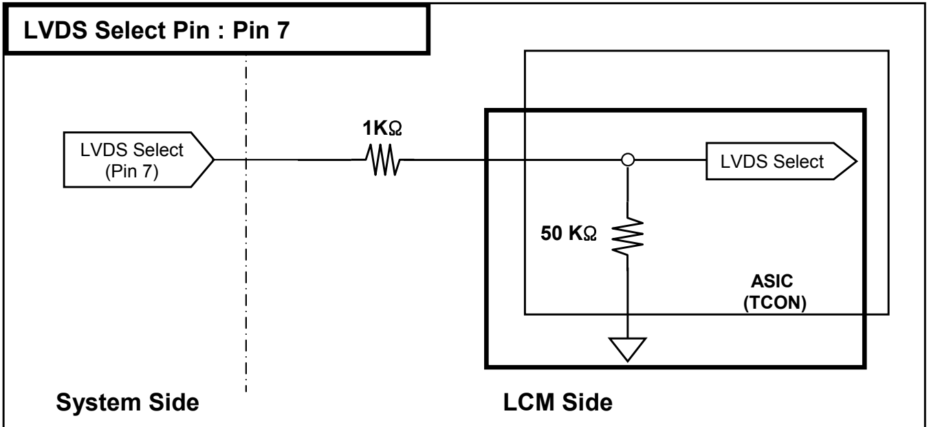
Circuit Block Diagram of LVDS Format Selection pin
