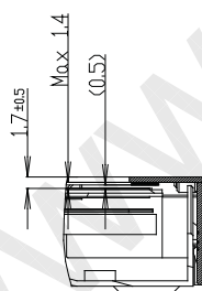
SECTION A-A SCALE 1/1
