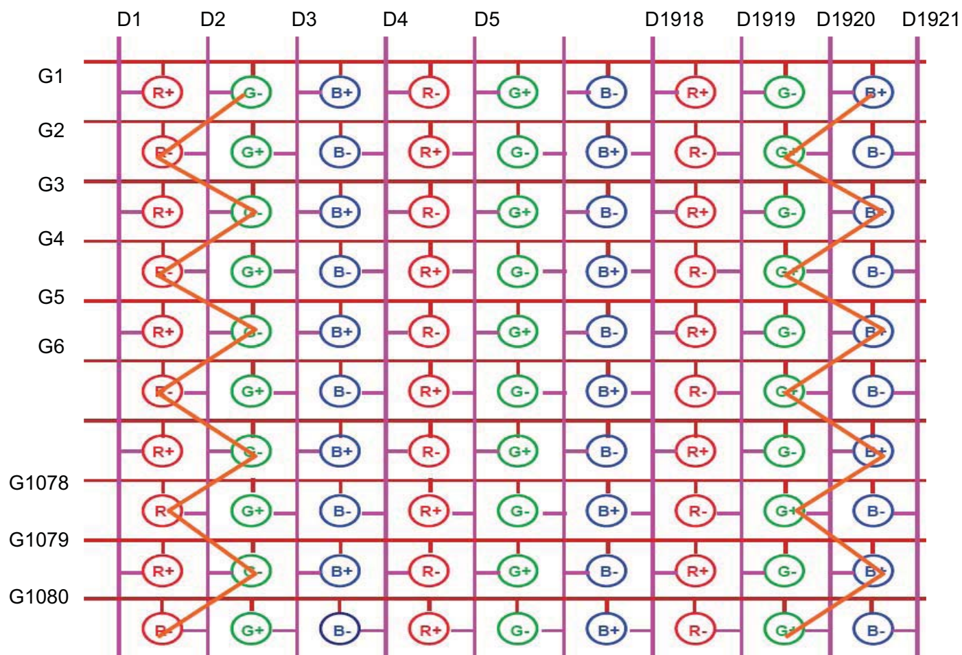
FIG. 5 Panel Pixel Structure
