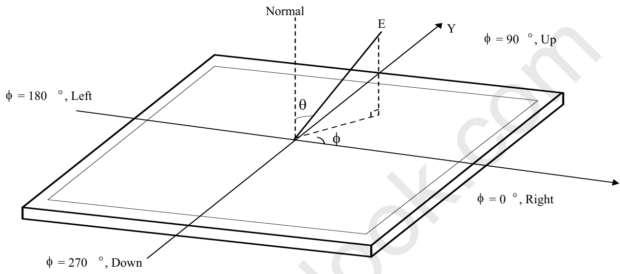
FIG.12 Viewing Angle
