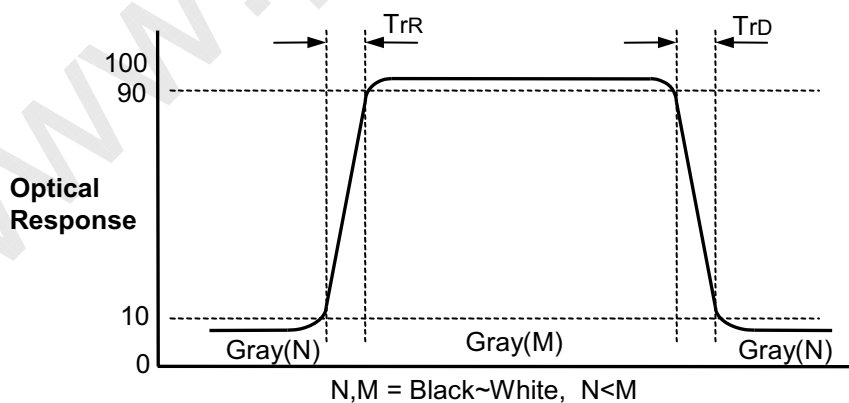
FIG. 11 Response Time
